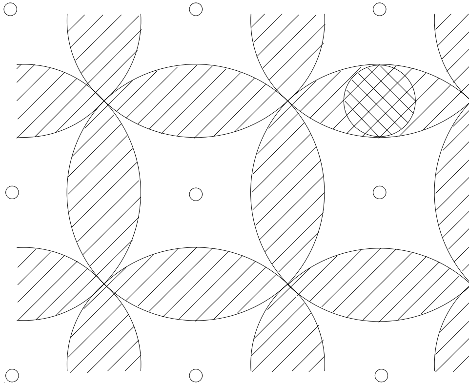
Figure 1. The covering multiplicity of the square lattice I_2 (small circles) is 2, since all points in the open lunes (shaded) are covered twice. An umbral circle is shown doubly-shaded.
