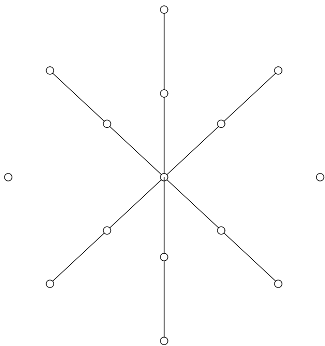
Fig. 3 Exclusion graph for E_7^* .
