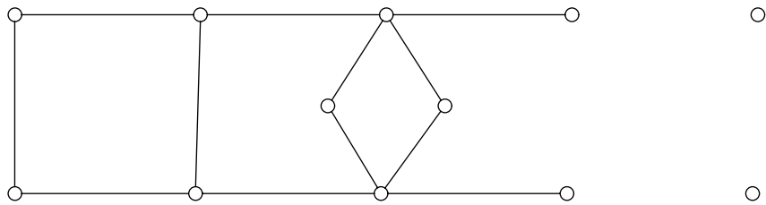
Fig. 2 Exclusion graph for A_4 .
