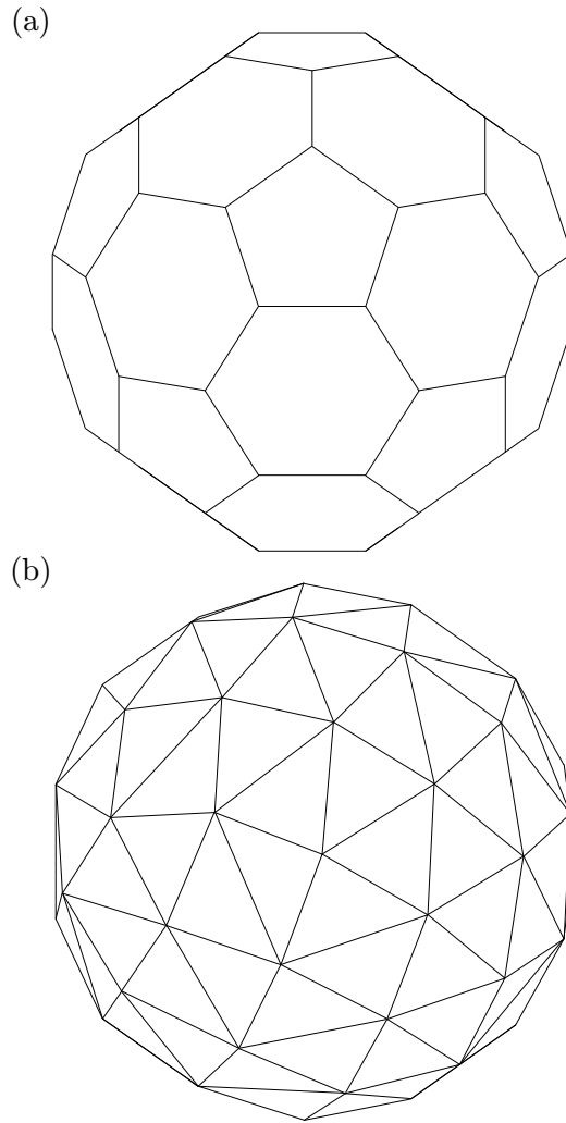
Figure 1: (a) The regular truncated icosahedron (or soccer ball), whose 60 vertices form a spherical 5-design. The Goethals-Seidel improved football [14], which forms a spherical 9-design, is almost indistinguishable from this. (b) Our 60-point spherical 10-design.
