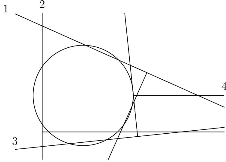
Figure 45: Enlargement of the central portion of a configuration of four lollipops with 40 intersections. Three of the lollipops are so large they appear as \bar{\Gamma} shapes. It seems unlikely, but it is true that because the lines numbered 1, 2, and 3 are actually circles, when the lines are extended, lines 1 and 2 will cross a second time, lines 1 and 3 will cross twice, and line 4 will cross line 1 a second time and will cross line 3 twice.
