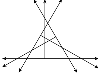
Figure 28: Three constrained long-legged \overline{T} 's can divide the plane into 19 regions. It is impossible to add a fourth \overline{T} that meets each of the first three in 4 points.
